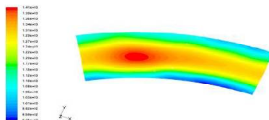
Fig 3.3 Temperature Contour For stage 3 RPF = 0.12
