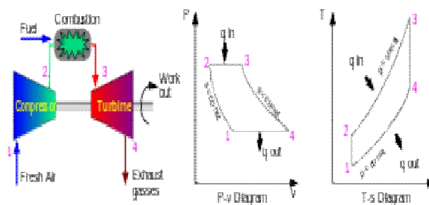
Fig 1.10 Idealized Brayton Cycle
