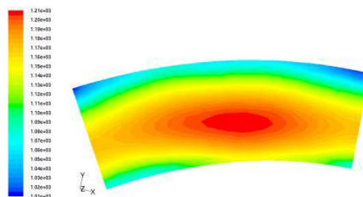
Fig 3.1 Temperature Contour For stage 1 RPF = 0.7
